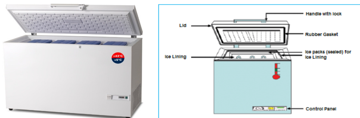
Figure 24. Ice-Lined Refrigerator
